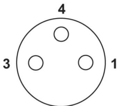
Pin assignment
