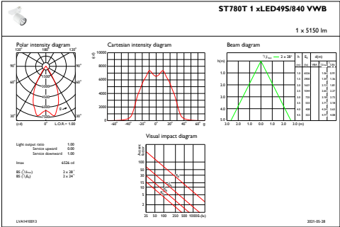
IFAS1_ST780T1xLED49S840VWB
