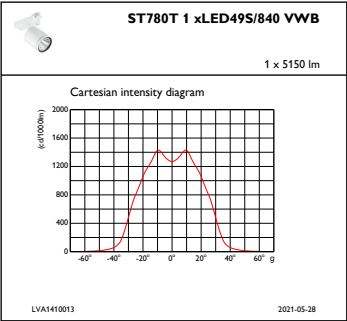
IFCC1_ST780T1xLED49S840VWB
