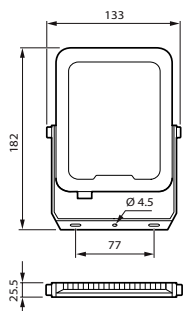
BVP164 LED36/840 PSU 30W SWB CE
