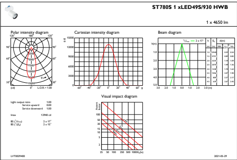
IFAS1_ST780S1xLED49S930HWB
