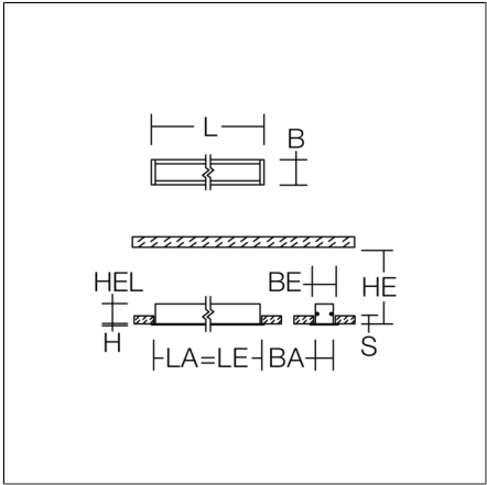
Recessed ceiling and wall luminaires 4051859286769 L 861, B 71, H 2 Recessed ceiling mounting, wall (recessed) deep black, matt (RAL 9005)
