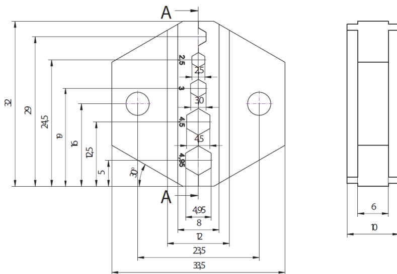
Dimensional drawing crimping die
