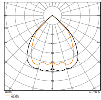
LN INV D 1200 P 40W 940 BK 800mA
