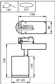
ST780T 49S/830 DIA-VLC HOVL-H BK
