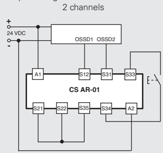
Input configuration with manual start 2 channels
