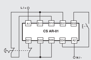
Input configuration with manual start 2 channels
