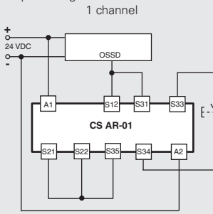
Input configuration with manual start 1 channel
