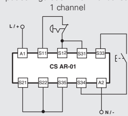
Input configuration with manual start 1 channel
