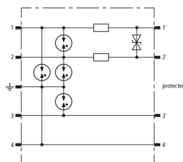
Basic circuit diagram BXT M2 BD S EX 24
