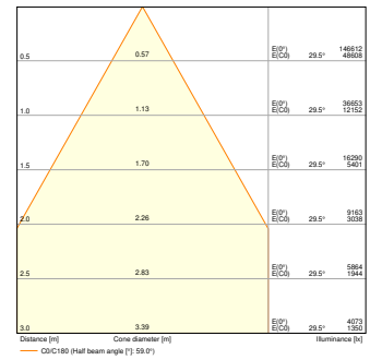
HB P 200W 865 70DEG IP66 PS - REFRACTOR
