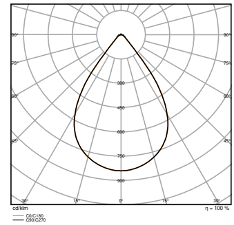
HB P 173W 865 70DEG IP66 PS
