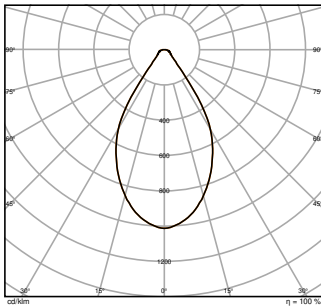
HB P 200W 865 70DEG IP66 PS
