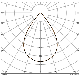
HB P 200W 865 70DEG IP66 PS set to 173W
