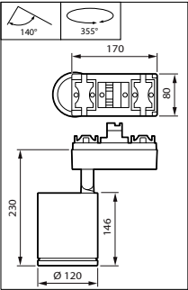
ST780S 49S/840 DIA-VLC VWB FG WH
