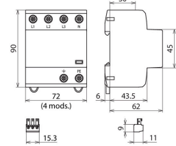
Dimension drawing DSH TNS 255 FM
