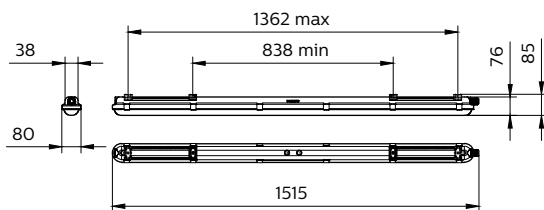
WT120C G2 LED40S/840 WIA TW3 L1200
