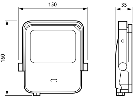
BVP154 LED20/830 PSU 20W VWB MDU CE
