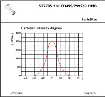
IFCC1_ST770S1xLED49SPW930HMB
