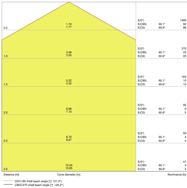
SF CIRCULAR 350 18W 3000K S IP44
