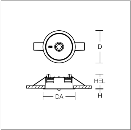
Recessed ceiling luminaires, Ceiling luminaires 4051859721277 D 135, H 2 Ceiling mounting, Recessed ceiling mounting white
