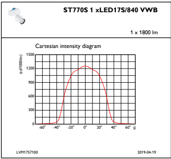
IFCC1_ST770S1xLED17S840VWB
