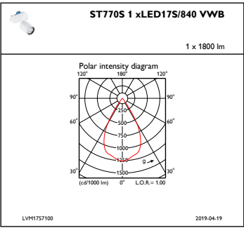
IFPC1_ST770S1xLED17S840VWB
