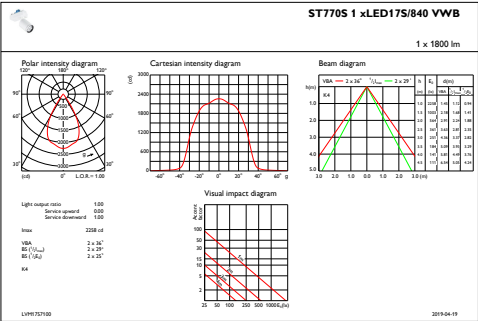
IFAS1_ST770S1xLED17S840VWB
