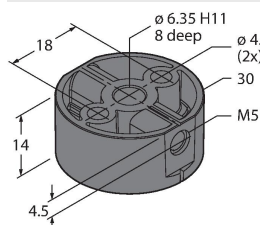
P2-RI-QR20
