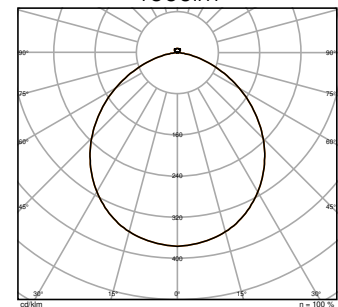
SF C 500 42W BLACK FRAME 3000lm
