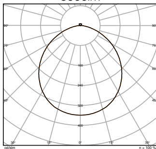
SF C 500 19W BLACK FRAME 1300lm
