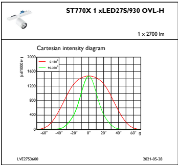
IFCC1_ST770X1xLED27S930OVL-H
