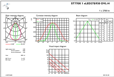
IFAS1_ST770X1xLED27S930OVL-H
