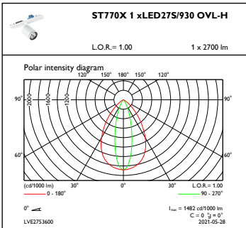
OFPC1_ST770X1xLED27S930OVL-H
