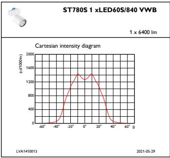
IFCC1_ST780S1xLED60S840VWB
