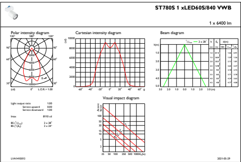
IFAS1_ST780S1xLED60S840VWB
