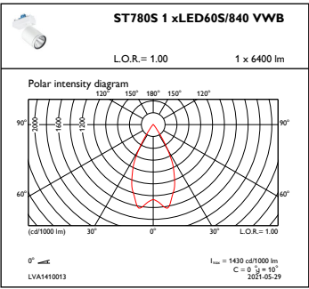
OFPC1_ST780S1xLED60S840VWB
