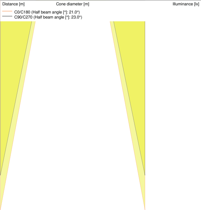
TRACK SP D85 35W4000K 90RA NFL GY
