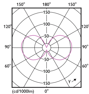
Light Distribution Diagram - CorePro LEDCandleND6.5-60W B35 E14840CLG
