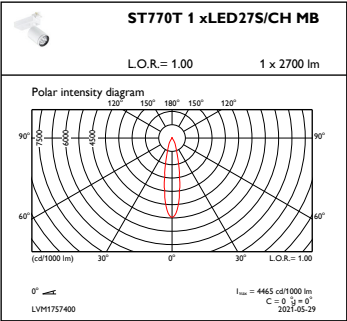
OFPC1_ST770T1xLED27SCHMB
