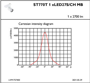
IFCC1_ST770T1xLED27SCHMB
