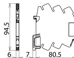
Dimension drawing DCO SD2 ME 48
