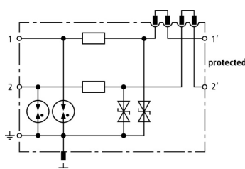
Basic circuit diagram DCO SD2 ME 48
