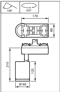
ST770S 17S/830 PSU MB FG WH
