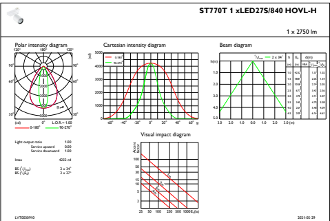
IFAS1_ST770T1xLED27S840HOVL-H
