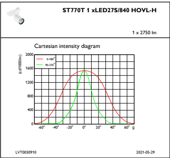
IFCC1_ST770T1xLED27S840HOVL-H
