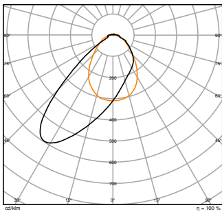
TRUSYS FLEX P 70W 865 WW CL WT DALI
