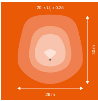
Floodlight Performance 150W ASYM 55x110 simplified isolux diagram
