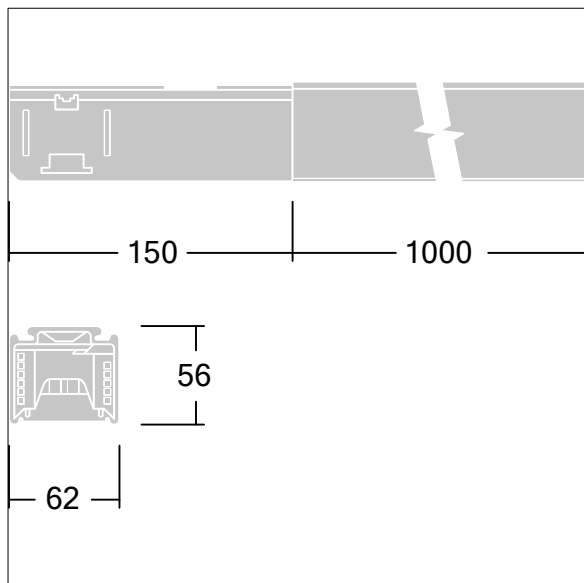
TL_CONTUS_M_Flexible_electrical_feed_out.wmf
