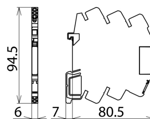
Dimension drawing DCO SD2 MD 48
