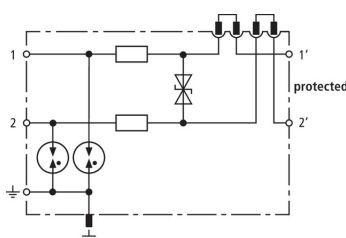
Basic circuit diagram DCO SD2 MD 48
