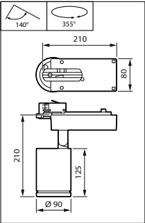
ST770T 27S/PC930 PSU MB FG SI
