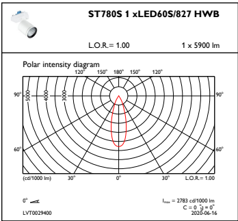
OFPC1_ST780S1xLED60S827HWB
