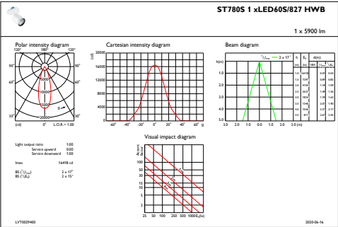
IFAS1_ST780S1xLED60S827HWB
