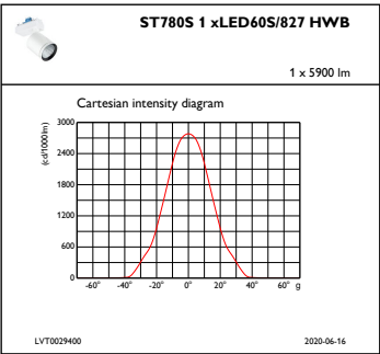
IFCC1_ST780S1xLED60S827HWB
