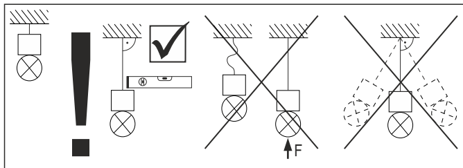
Opal
