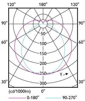
Light Distribution Diagram - MAS LEDtube 600mm HO 7.6W830 T8
