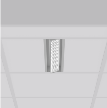
Recessed projectors 4051859937371 L 597, B 116, H 39
