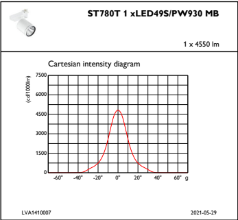
IFCC1_ST780T1xLED49SPW930MB
