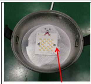
Figure3 Remove the screws
