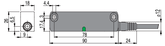
ST H••••N• sensor with cable
