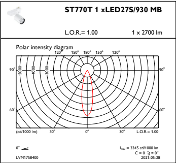
OFPC1_ST770T1xLED27S930MB
