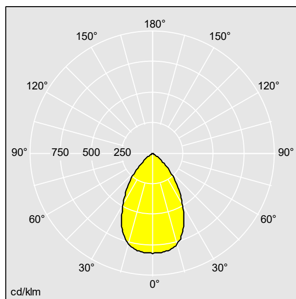
TLG_CHAL3_200_1400-830_EHF_RSB.ltd
