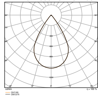
HB P 150W 865 70DEG IP66 PS - REFLECTOR
