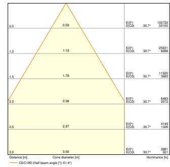
HB P 150W 865 70DEG IP66 PS - REFRACTOR
