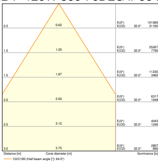
HB P 150W 865 70DEG IP66 PS - REFLECTOR
