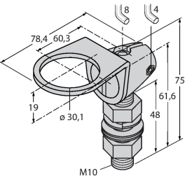
SMB30FAM10 3011185
