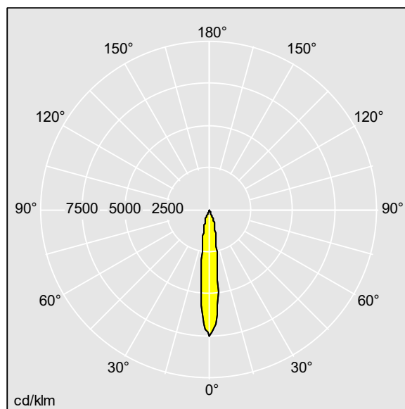
TLG_LE_1327_GRAFFITI_3600-940HE_SP.Idt
