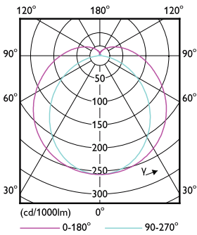
Light Distribution Diagram - MAS LEDtube 600mm HO 7.6W865 T8
