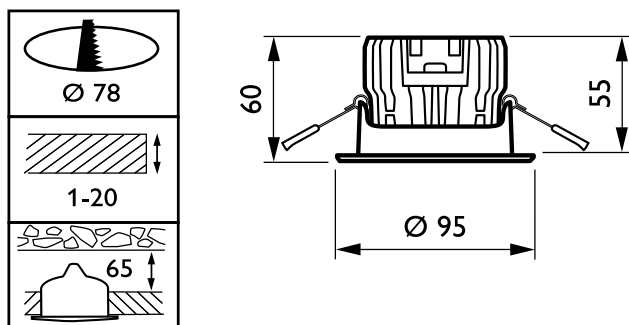
RS140B LED9-32-/830 PSR PI6 ALU
