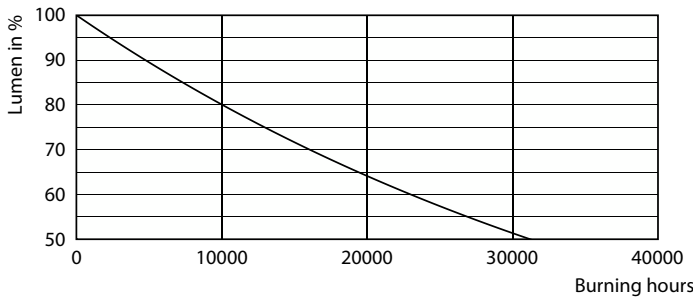
Lumen Maintenance Diagram - LEDbulb ND 4.9-40W A60 E27 840 2CT
