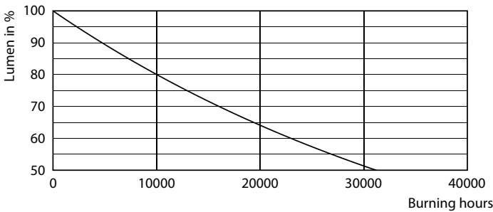
Lumen Maintenance Diagram - LED classic 48W A60 E27 825 GOLD NDSRT4
