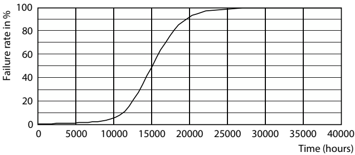
Life Expectancy Diagram - LED classic 48W A60 E27 825 GOLD NDSRT4
