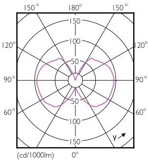
Light Distribution Diagram - LED classic 48W A60 E27 825 GOLD NDSRT4
